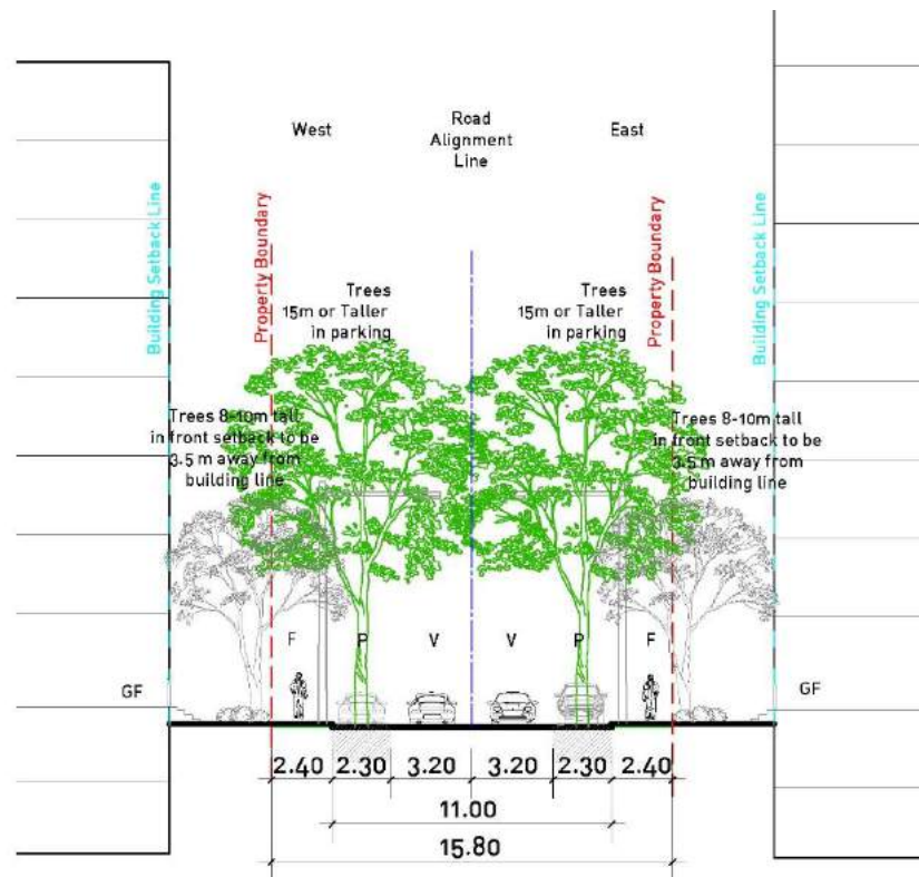
NSR 5 - 15.8 M WIDE STREET
