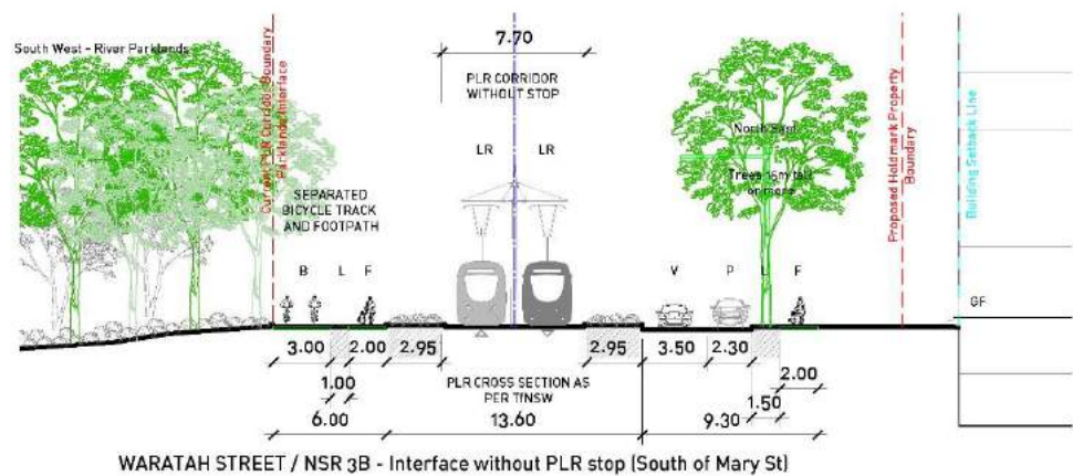
Figure 15 – Type 7 Local Street (NSR 3B in areas without Stop)
